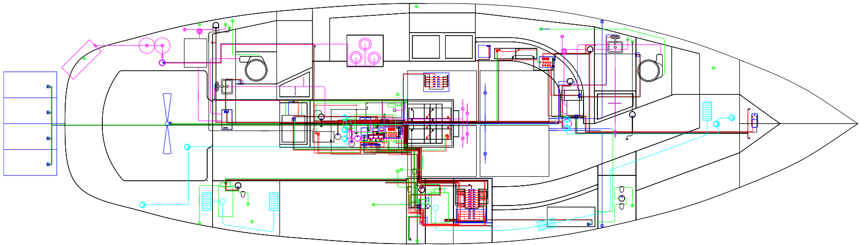
GENERAL ASSEMBLY ~ ELECTRICAL, WATER, WASTE, LPG, SHORE POWER, AIR CONDITIONING, DIESEL and NAVIGATION SYSTEMS
