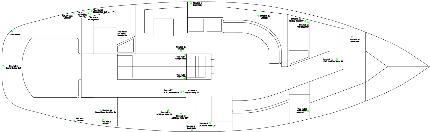
SEA COCK, THRU HULL I.D. AND AWL OUTLET LOCATIONS
